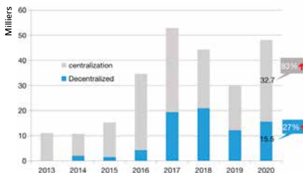
Fig. 2 - China's newly installed capacity situation (GW) (Source: CPIA).
