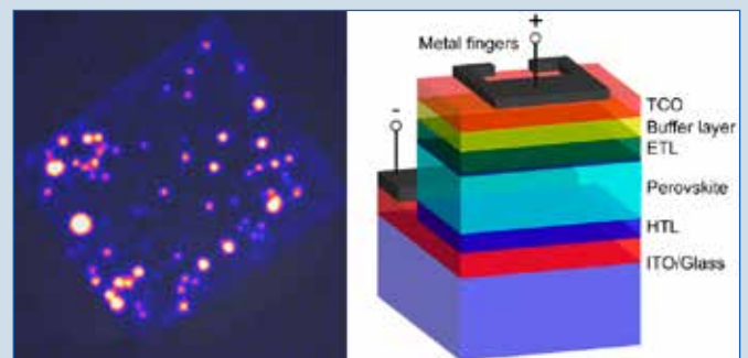
Fig. 5 - (Left) Lock-in thermography image of a semi-transparent perovskite solar cell exposed to a reverse bias of -3V showing hot-spot/shunt formation over the entire cell area. (Right) Schematic of a semi-transparent perovskite solar cell architecture, such as it would be used in a tandem cell configuration (with the Si bottom cell replacing ITO/Glass) (Source: EPFL/CSEM).
