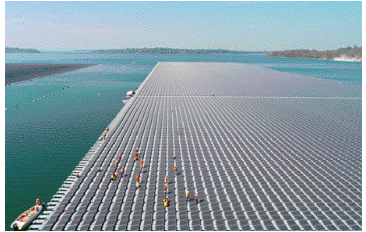
Fig. 1 - The 45 MW world's largest floating PV system, as part of the Hydro-Floating Solar Hybrid Project at Sirindhorn Dam, operated by the Electricity Generating Authority of Thailand (EGAT). This project will hybridize the FPVs with the hydropower dam to increase efficiency of the system (Photo: EGAT).
