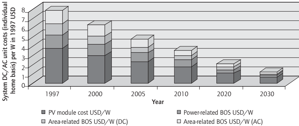
Figure 27 Cost Development and Indicators for Photovoltaic Systems
