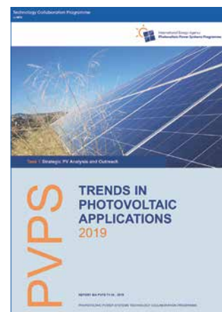
Fig. 2 – PVPS Report: Trends in Photovoltaic Applications – Survey Report of Selected IEA Countries between 1992-2018; Report IEA PVPS T1-36:2019.
