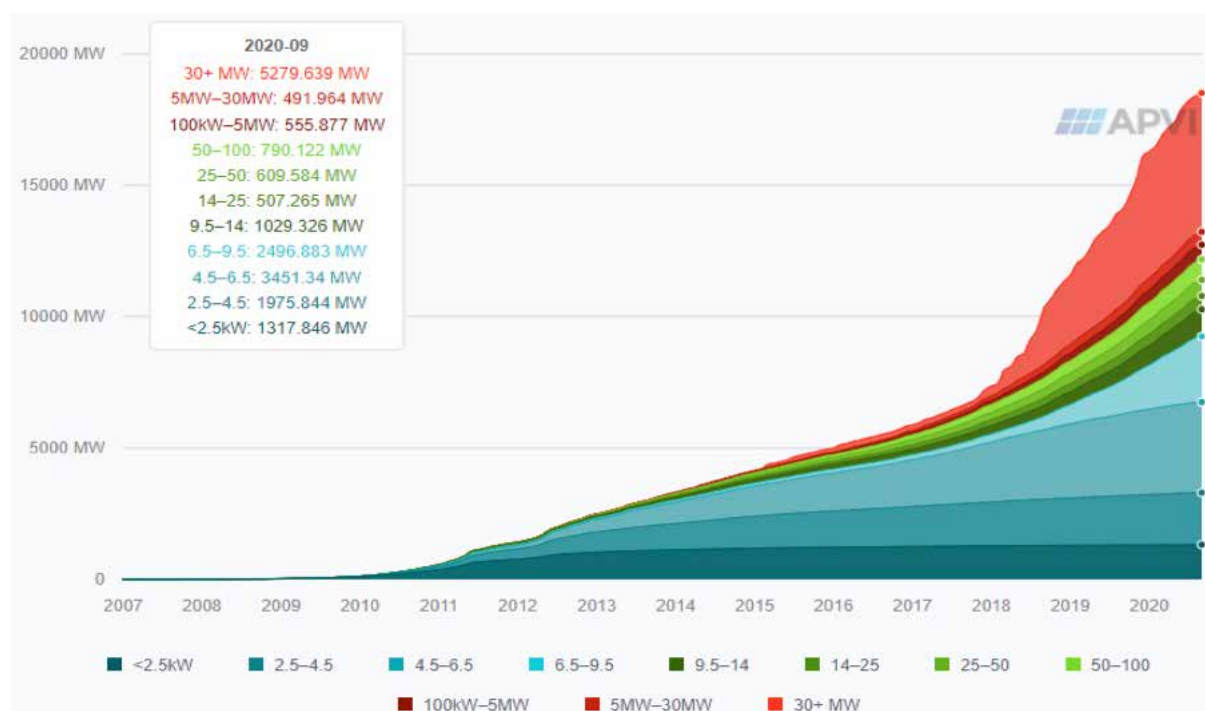
Fig. 2 - Cumulative installed capacity by system size to end of September 2020.
