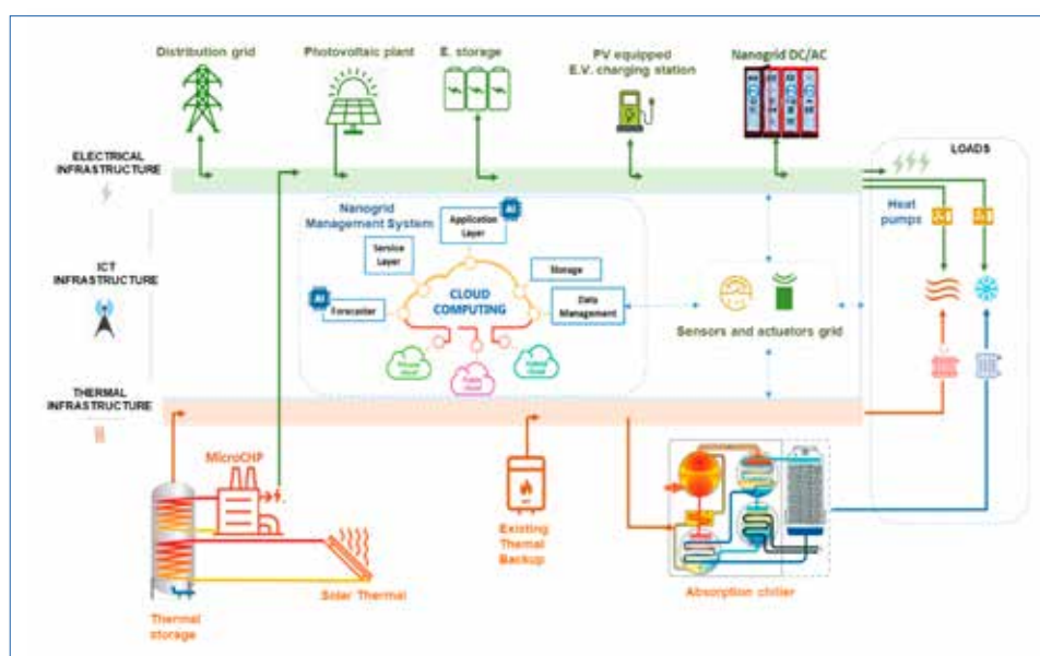
Fig. 3 - ENEA experimental multivector smart nanogrid layout.
