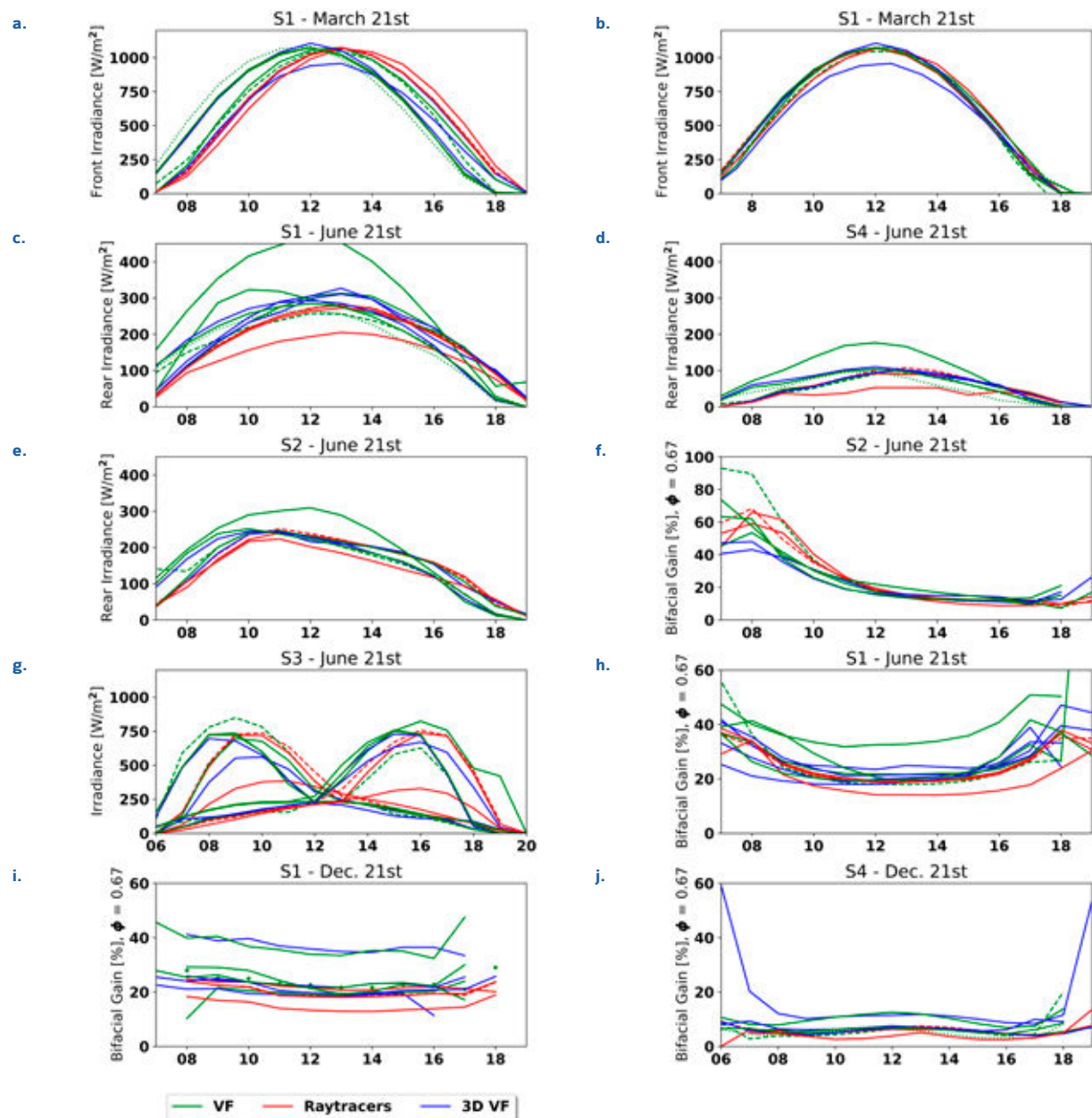
Fig. 2 - Example of modelling results run by ST1.2 experts for scenarios (S1-S4). The three model classes are denoted by colour: view factor models (green), raytracing models (red) and 3D VF and others (blue).
